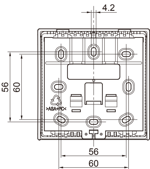
Rear view
